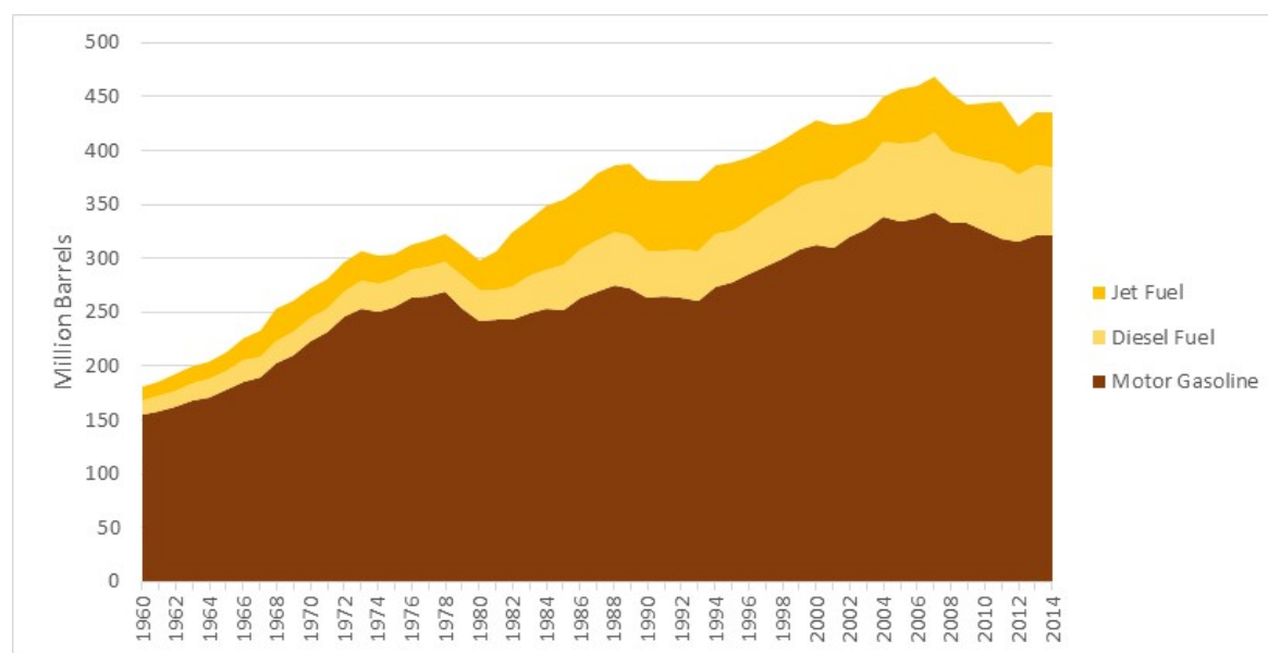
Figure 1: Northeast and Midatlantic Region Transportation Fuel Consumption.
