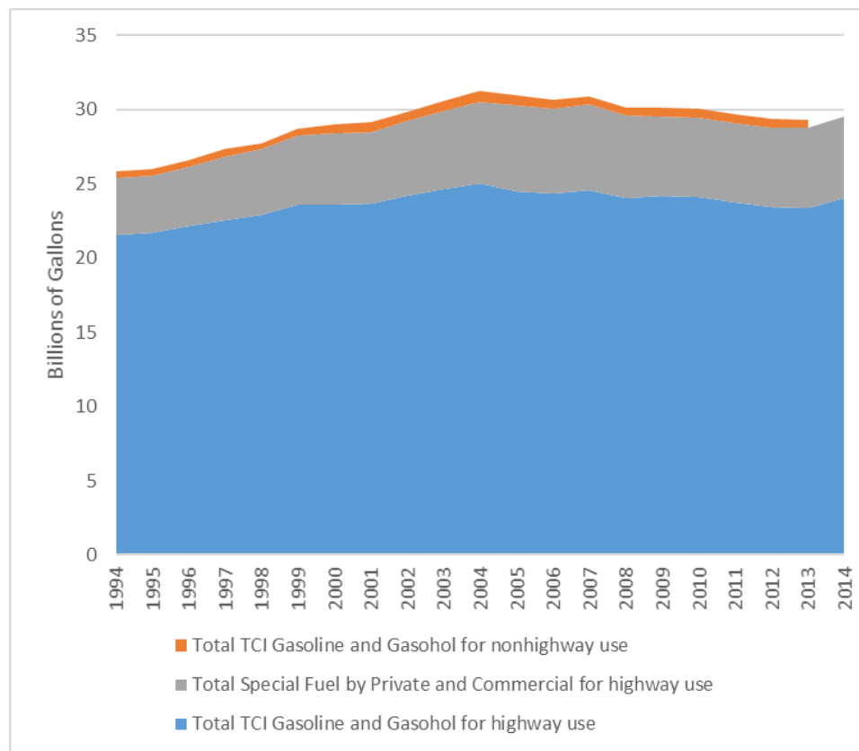
Figure 7: Motor Fuel Use Northeast and Mid-Atlantic 111
