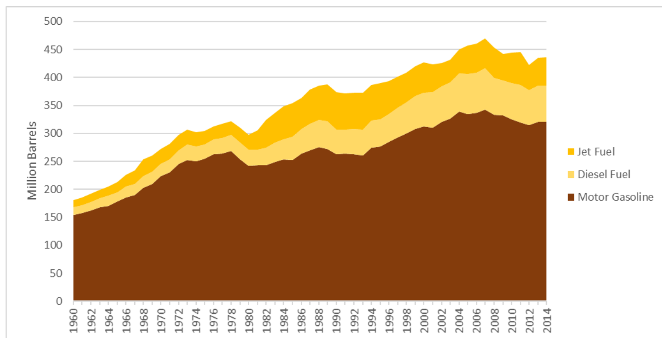
Figure 9 EIA SEDS Northeast and Mid-Atlantic Region Transportation Fuel Consumption 117
