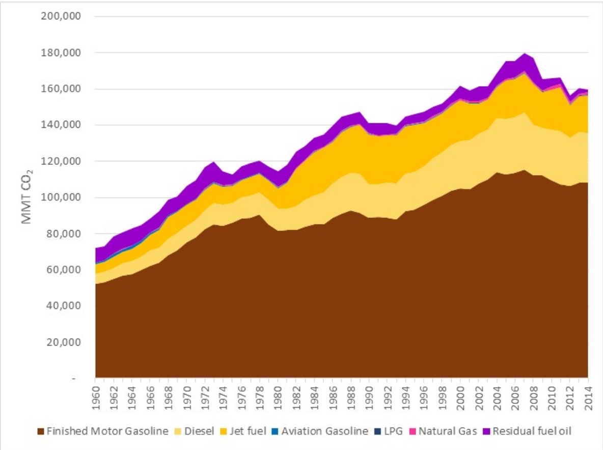
Figure 2: Northeast and Mid-Atlantic Transportation Emissions by Fossil Fuel Type.
