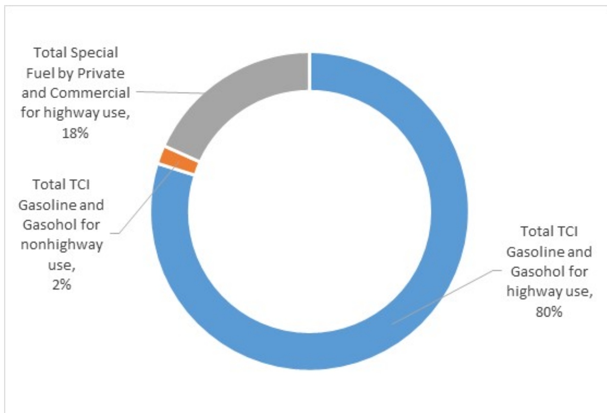
Figure 8: Motor Fuel Use in the Northeast and Mid-Atlantic, 2014. 112
