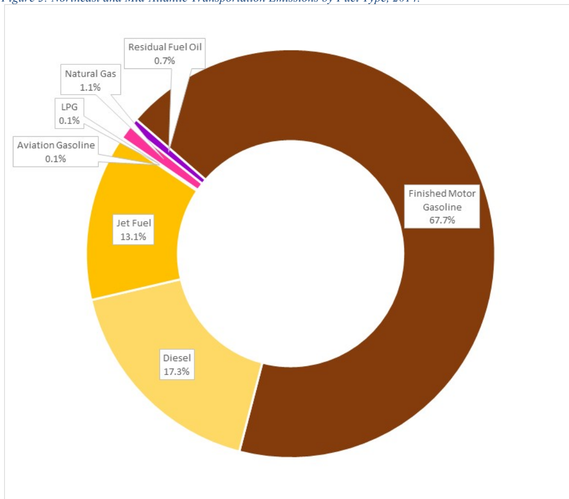
Figure 3: Northeast and Mid-Atlantic Transportation Emissions by Fuel Type, 2014.
